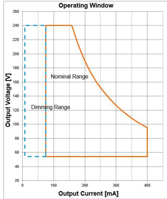
Operating Window ETI DALI 35/220-240/400 D LT2 L
